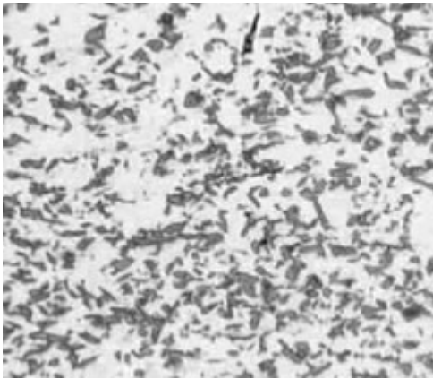
Cross sectional view of NiCom (NiSiC).
